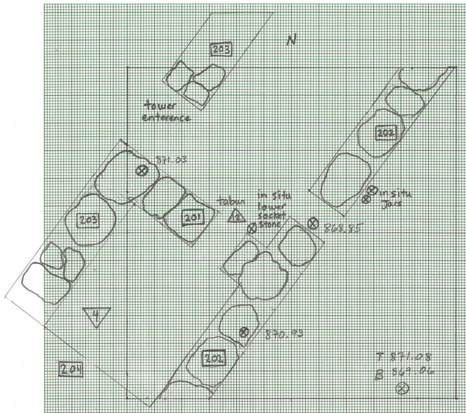
Figure 49: Top plan for X23 (by Mark Hassler).
